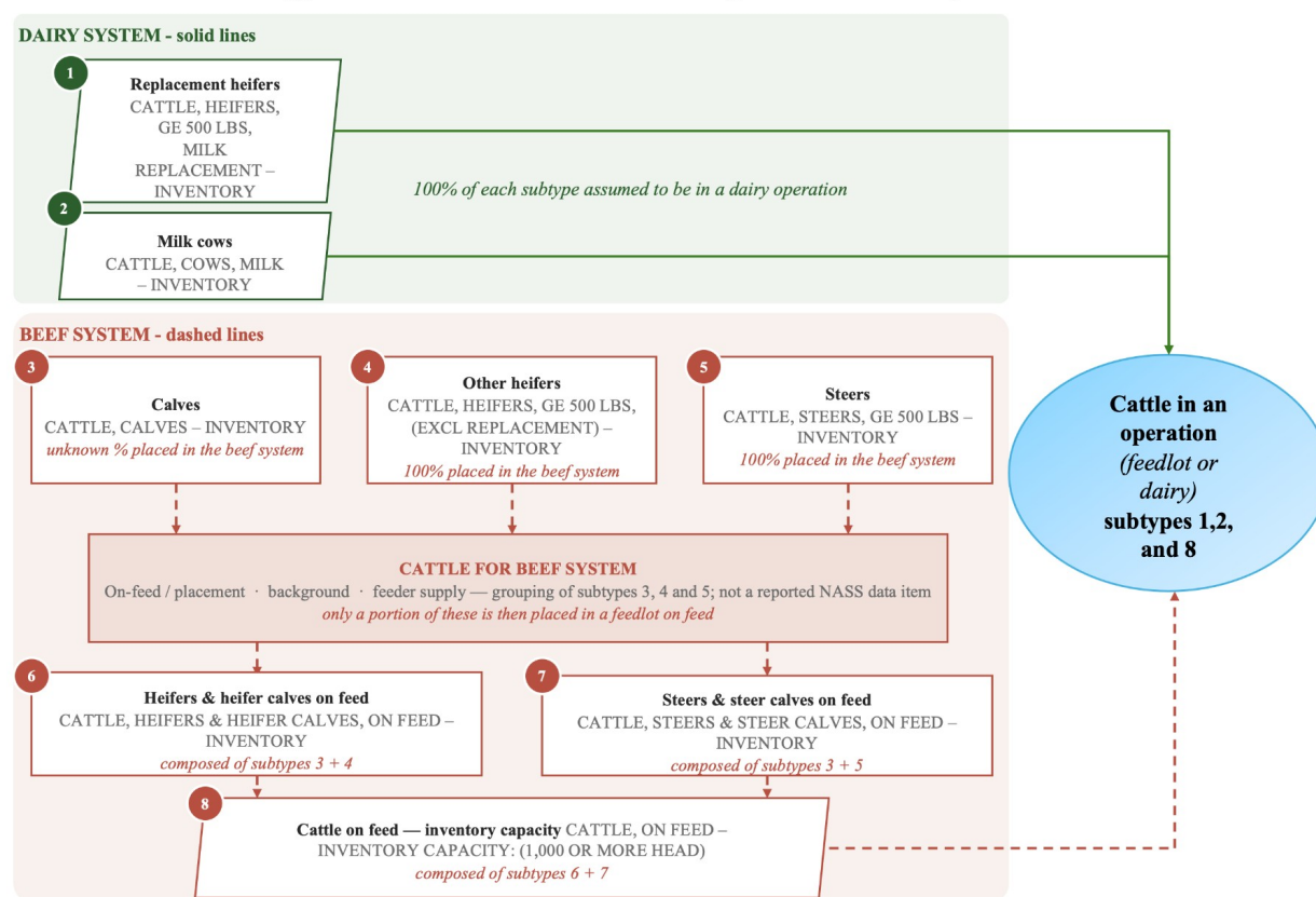
Figure 3 USDA NASS cattle subtypes considered to be in an operation. Parallelograms (subtypes 1, 2, and 8) are the subtypes carried forward and combined with Climate TRACE asset-level cattle operations to estimate state- and country-level emissions (circle); rectangles are intermediate subtypes. Solid lines represent the dairy system and dashed lines the beef system. Subtypes 1 and 2 — replacement heifers and milk cows — were assumed to be 100% in a dairy operation. On the beef side, all of subtypes 4 and 5 and an unknown percentage of subtype 3 enter the “Cattle for Beef System,” a grouping that is not itself a reported NASS Data Item; a portion of these are placed in a feedlot on feed and reported as subtypes 6 and 7, which together compose subtype 8. Subtype 8 is Cattle on feed – inventory capacity.
