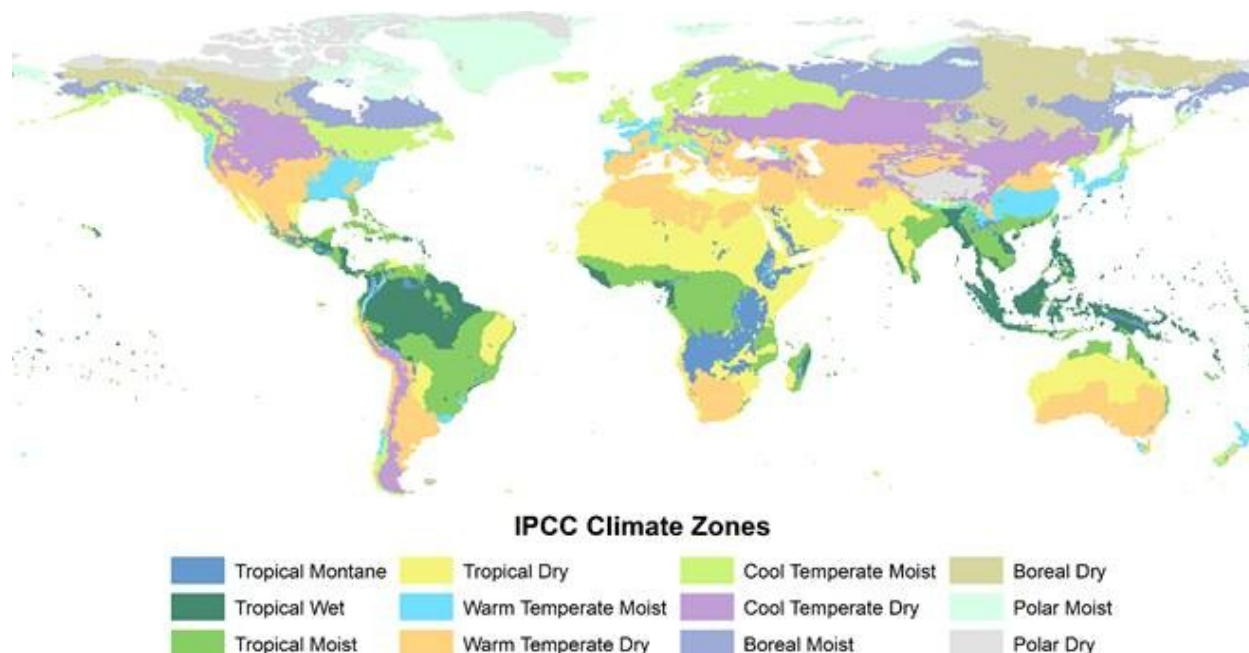
Figure 2 IPCC 2019 major climate zones identified (image taken from IPCC 2019 Chapter 3, volume 4; IPCC, 2019a).
