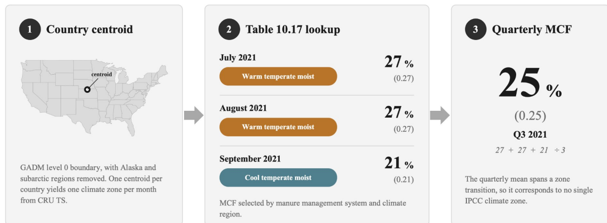
Figure 4 Illustrative example of the monthly-to-quarterly MCF derivation. Step 1 - a single GADM level 0 centroid per country gives one climate zone per month. Step 2 - each monthly climate zone selects an MCF from IPCC 2019 Table 10.17 by manure management system (from Table 10A.6 AWMS) and climate zone, applied separately to dairy and non-dairy cattle. Step 3 - the three monthly MCF values are averaged to a quarterly value - July, August, and September MCFs become quarter 3 MCF.
